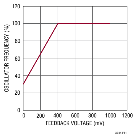
Figure 11. Frequency Foldback
